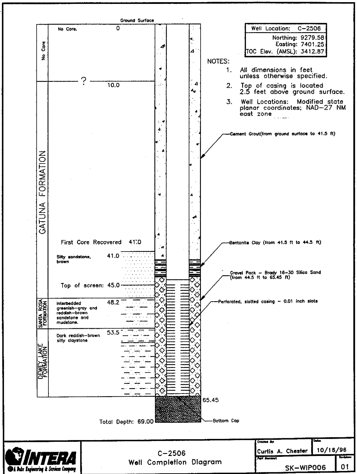
Figure 3.2 Well completion diagram - C-2506
