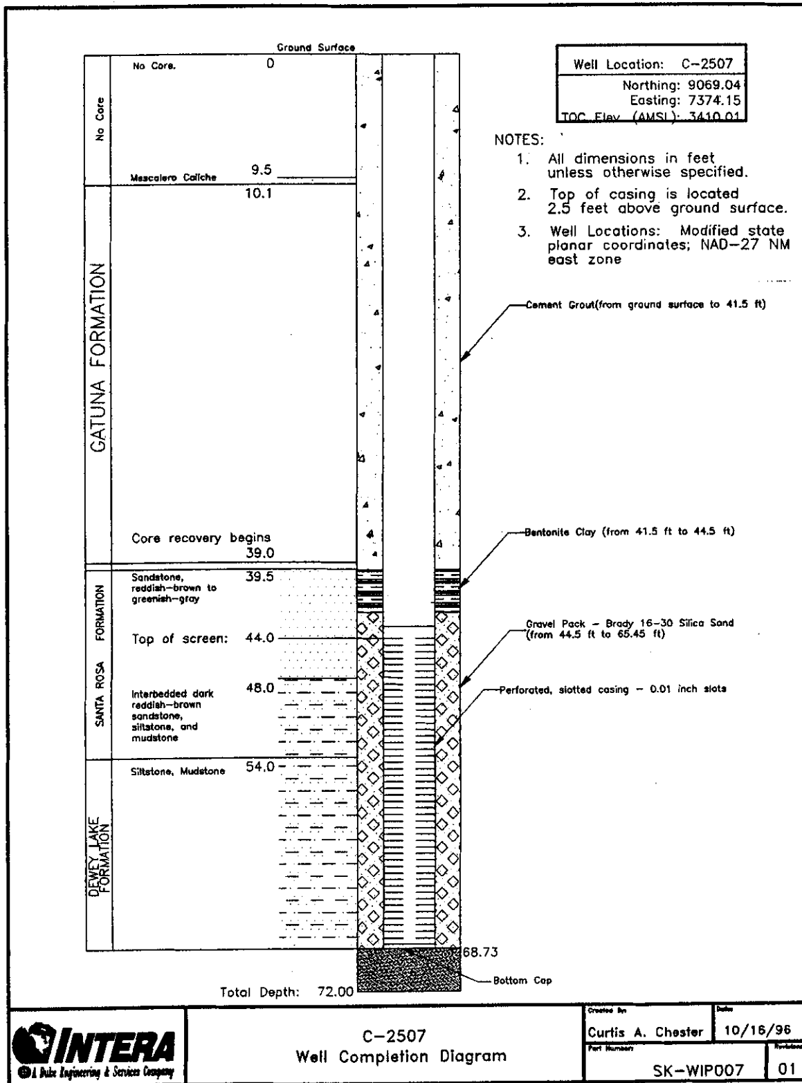
Figure 3.3 Well completion diagram - C-2507
