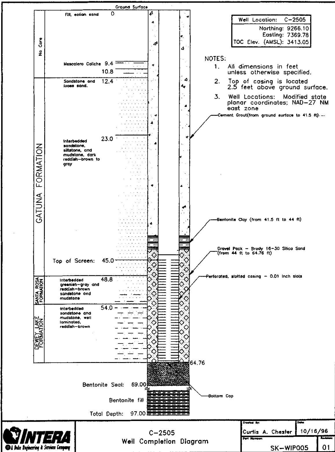
Figure 3.1 Well completion diagram - C-2505
